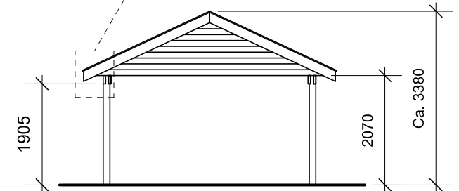
Front gavl
